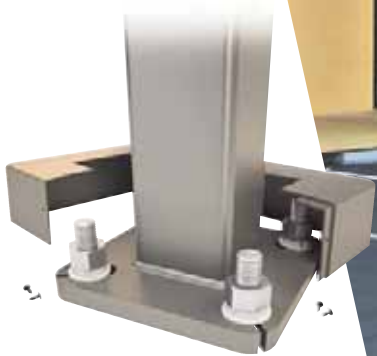
VSS Square Straight Steel Pole
