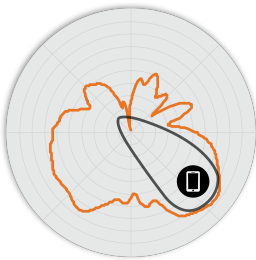
Figure 7. R670 6GHz Elevation Antenna Patterns
