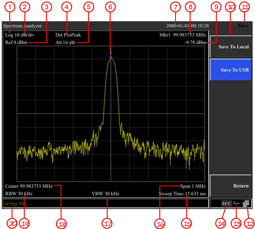
Figure 4-7 User interface
