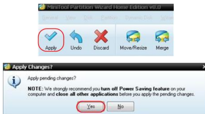
Figure 4- 16: Apply setting
