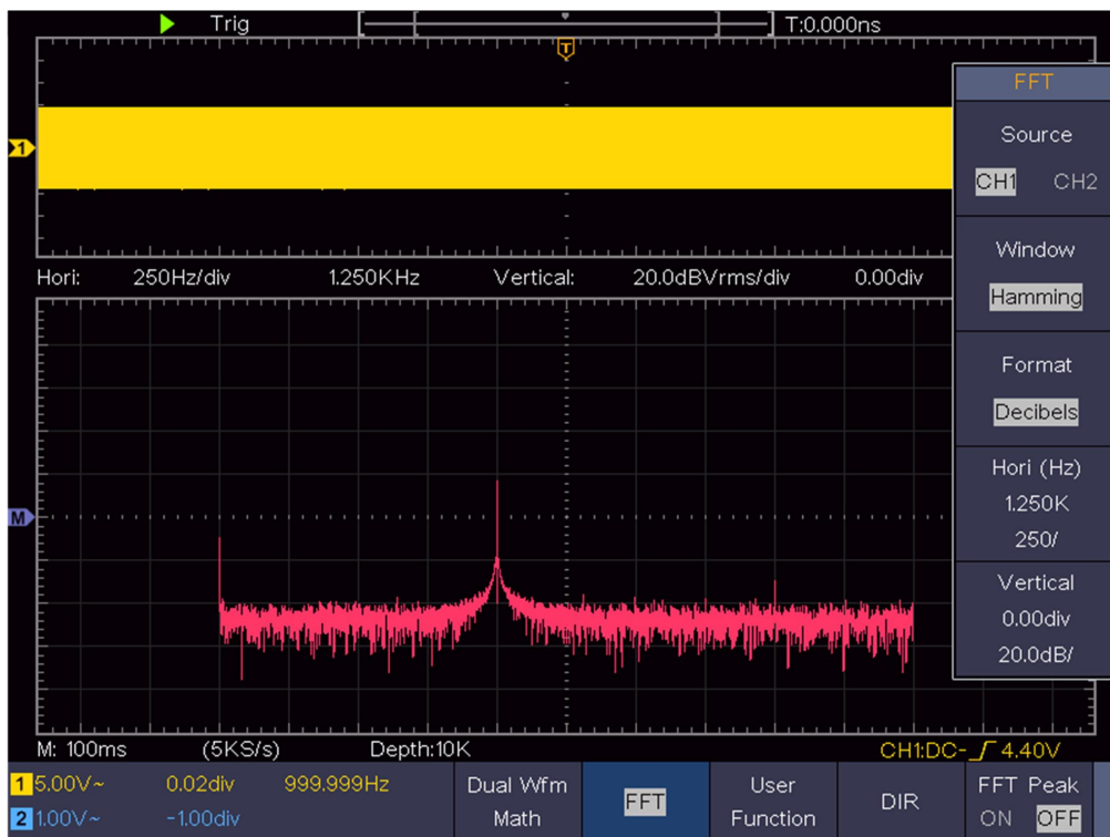
Figure 4- 1 Hamming window
