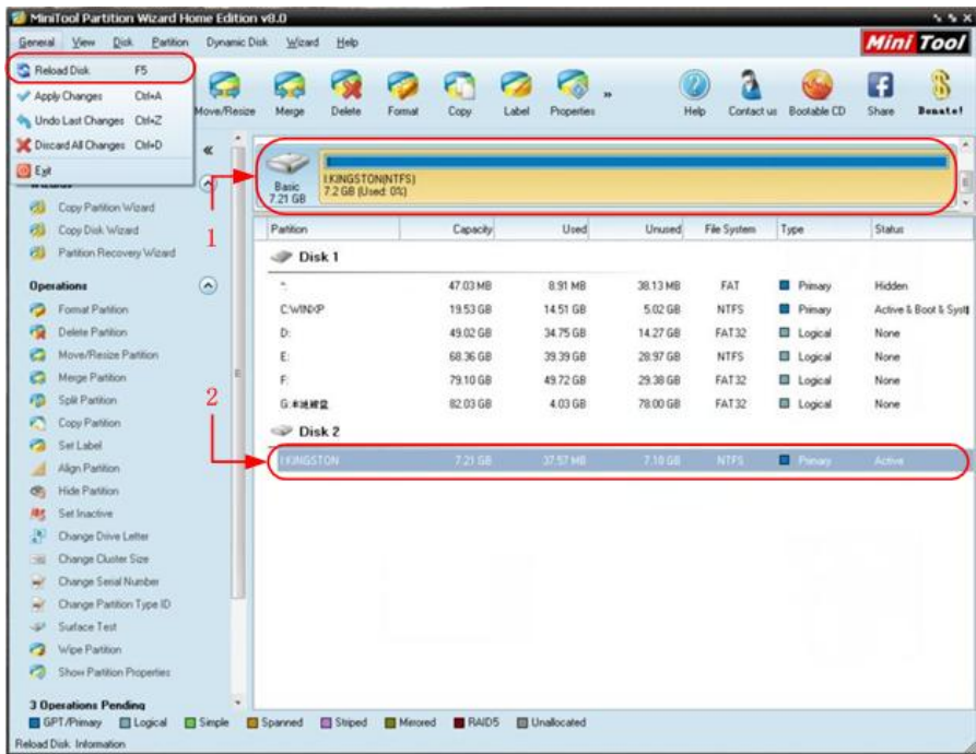
Figure 4- 13: Reload Disk
