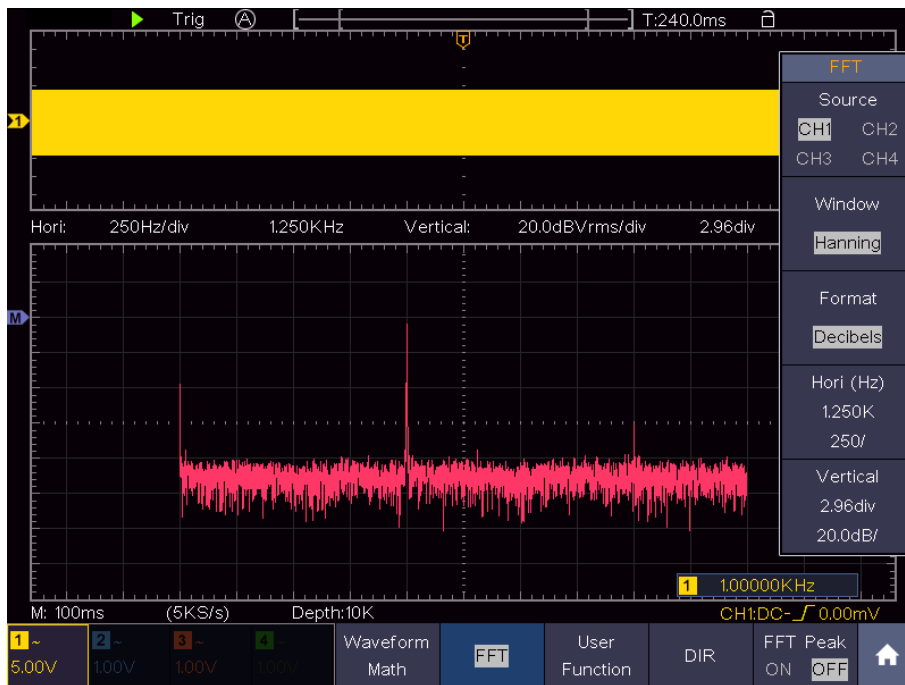
Figure 4-4 Hanning window
