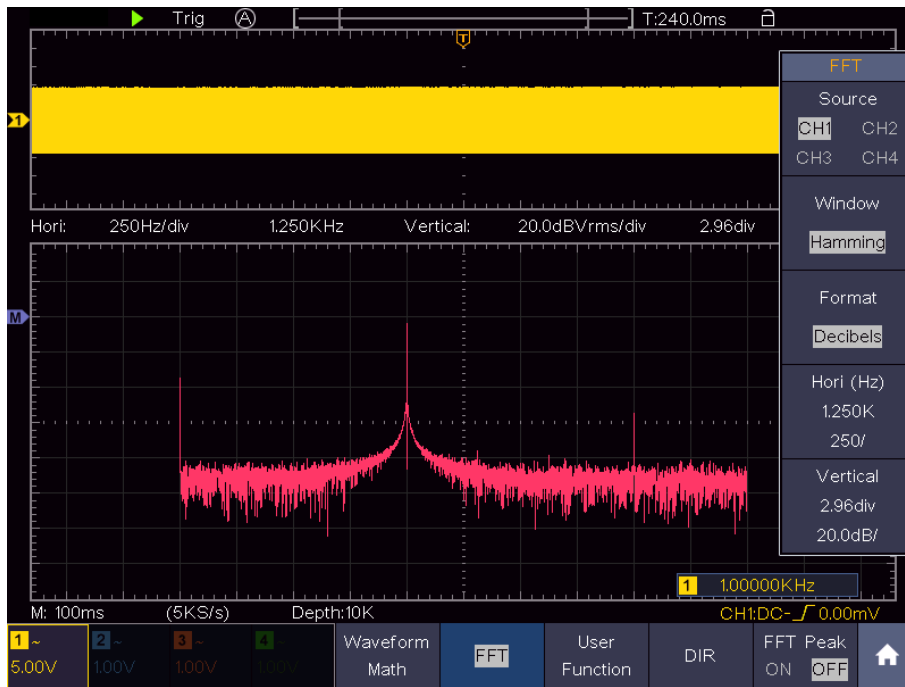
Figure 4-1 Hamming window
