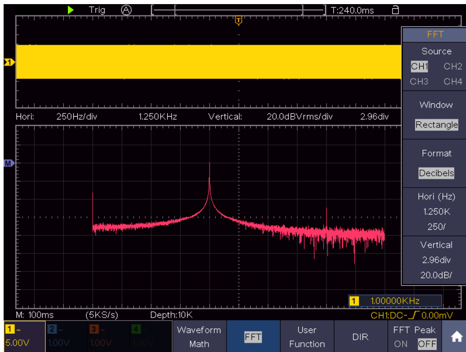
Figure 4-2 Rectangle window
