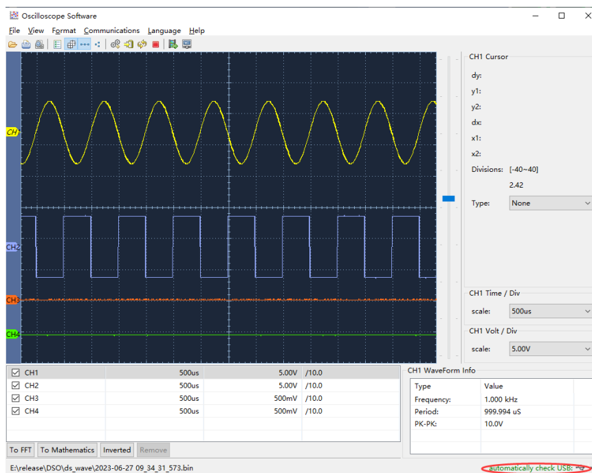
Figure 7-1 Connect with PC through USB port
