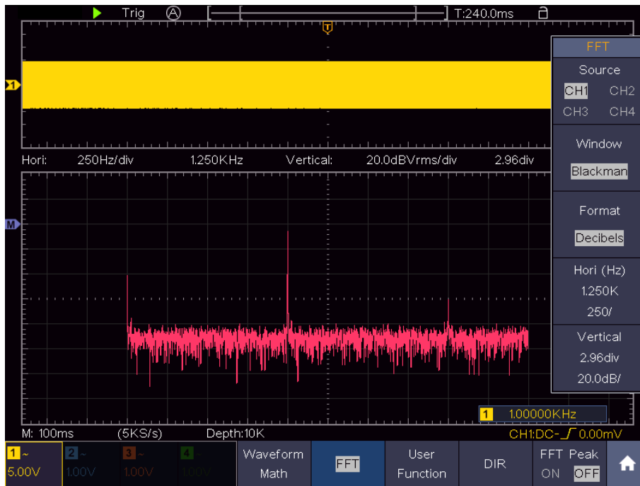
Figure 4-3 Blackman window
