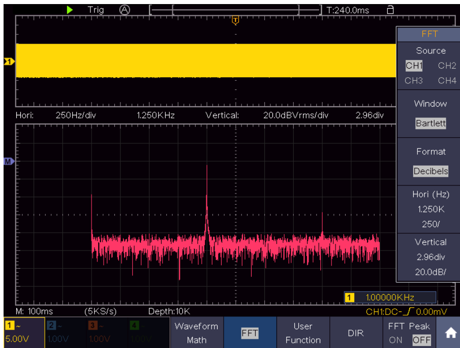
Figure 4-6 Bartlett window
