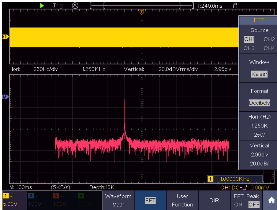
Figure 4-5 Kaiser window
