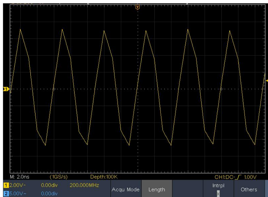
Linear interpolation
