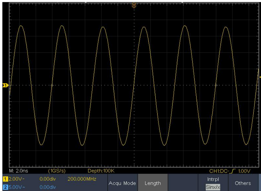
Sine(x)/x interpolation
