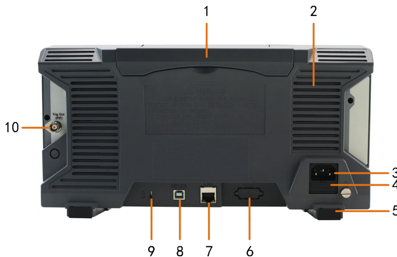
Figure 3-3 Rear Panel
