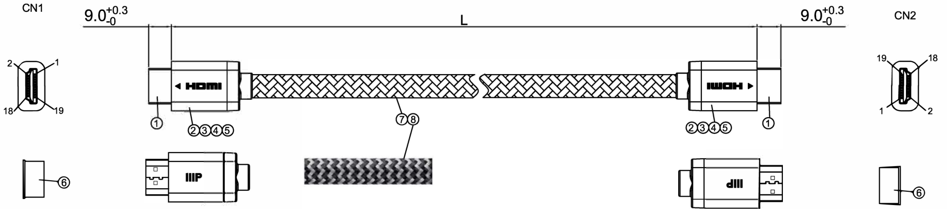
HDMI 19P/M MOLDING TYPE
