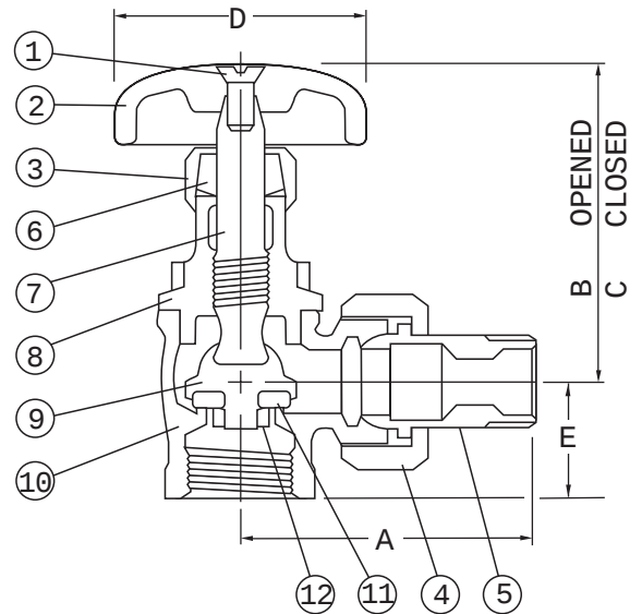
Pictured Model T-431 Cut-away
