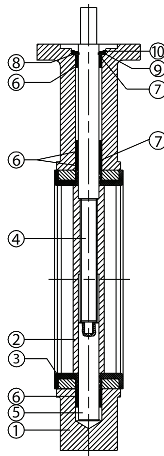
Pictured T-335AB, T-337AB Body, cut-away side view
