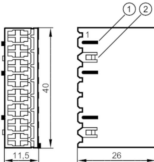
Figure shows contact housing with closed cover View on contact plug-in side
