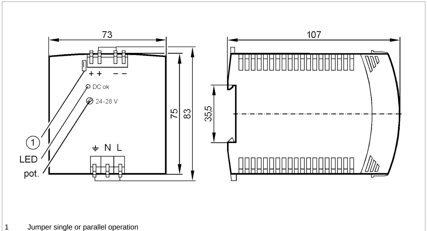
1 Jumper single or parallel operation
