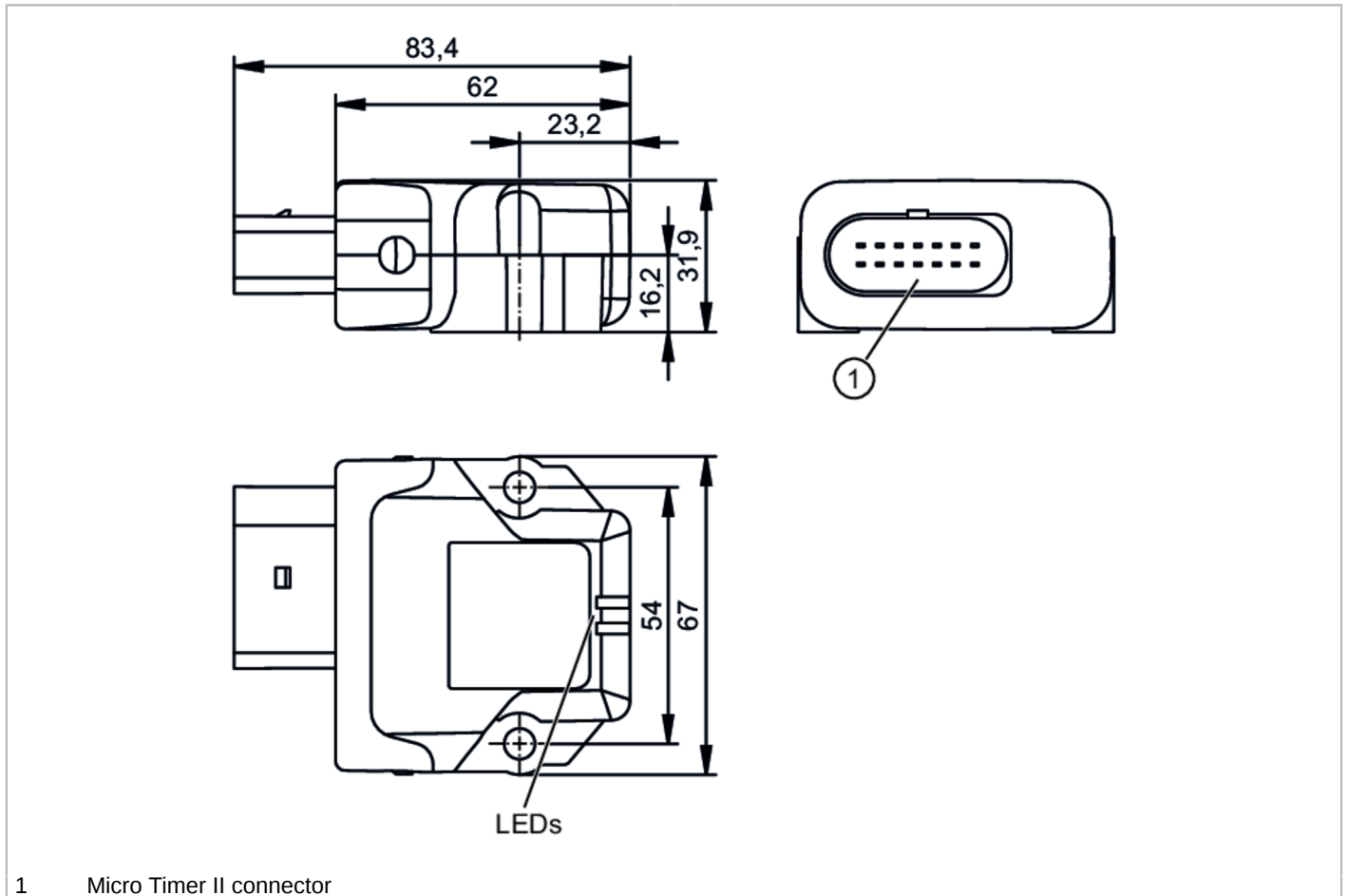
1 Micro Timer II connector
