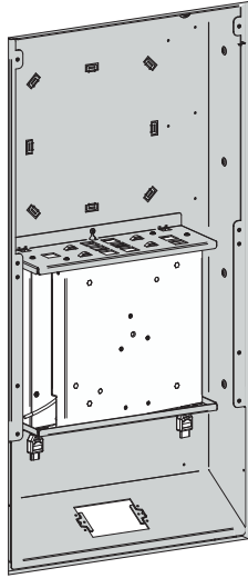
LP-TBRT Retractors (Ordered separately.)
