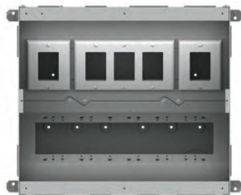
Plate Configuration 1-3-1
