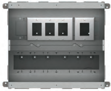
Plate Configuration 6-0
