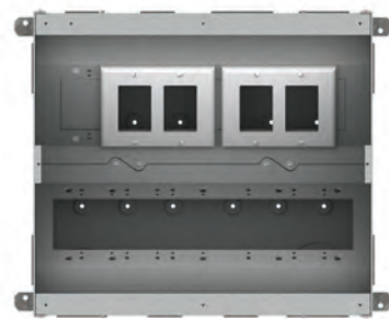
Plate Configuration 3-2
