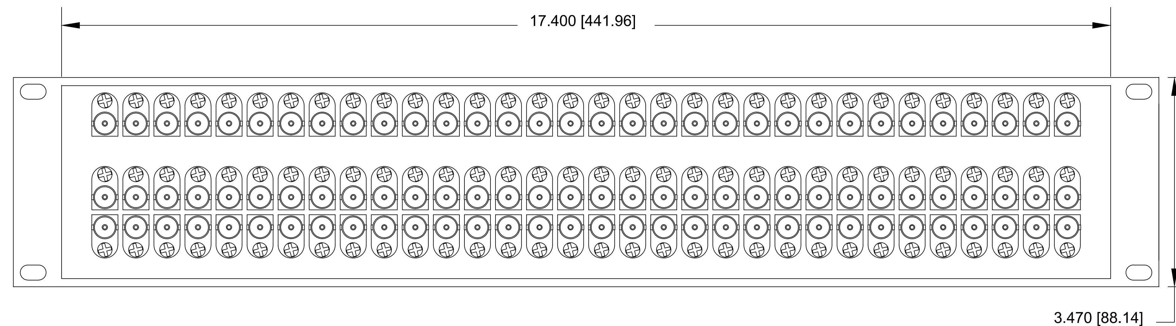
REAR VIEW
