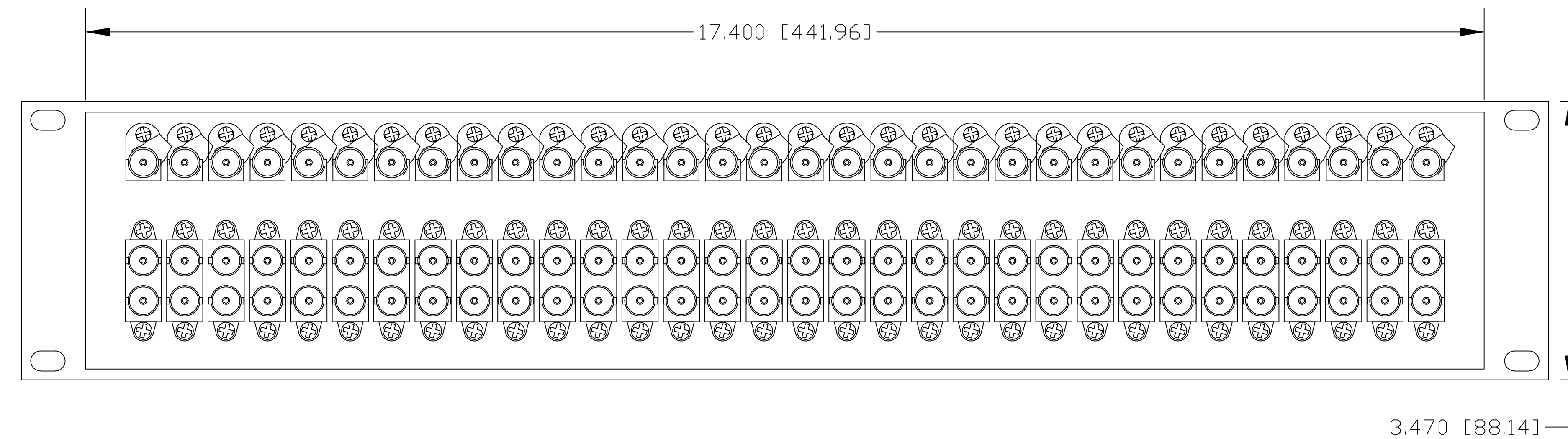
REAR VIEW
