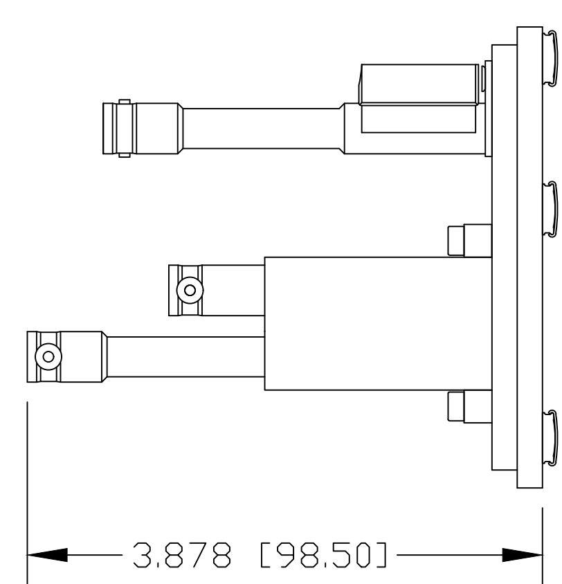
SIDE VIEW
