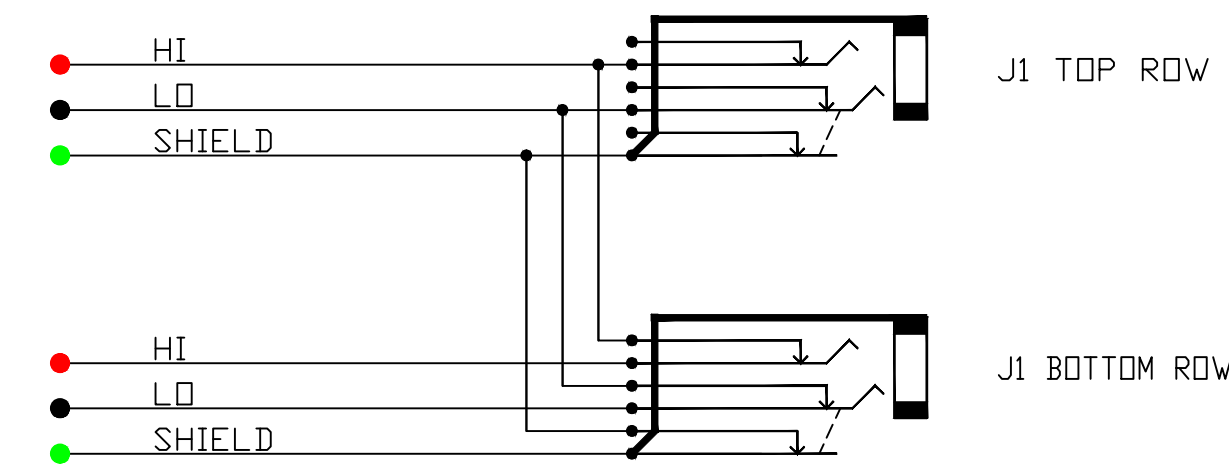
SCHEMATIC HALF-NORMALIZED SWITCHED GND VIEW
