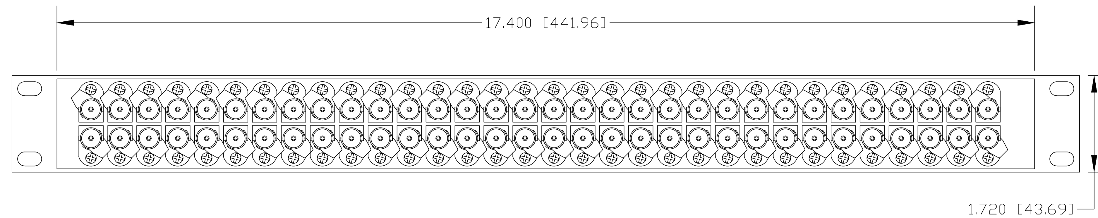
REAR VIEW
