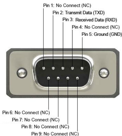
RS232 Pinout
