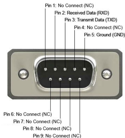
RS232 Pinout
