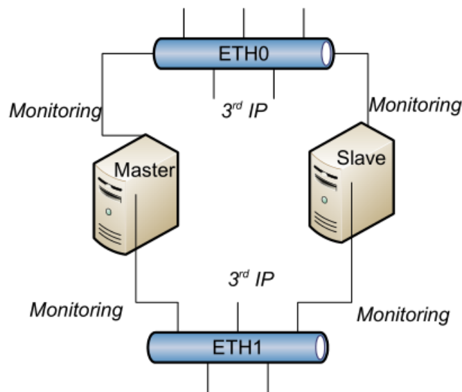
FIG. 54 Connection Diagram
