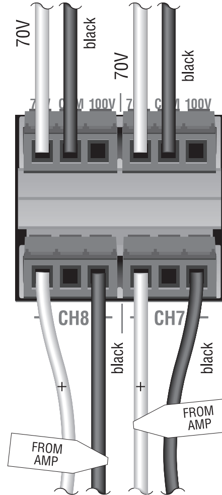
Figure 1. 70V Output
