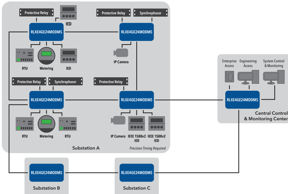
Electrical Substation SCADA Network using RLXE4GE24MODMS
