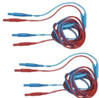
Doble-wire test lead 3 m (10 / 25 A) U1/I1 WAPRZ003DZBBU111 U2/I2 WAPRZ003DZBBU212
