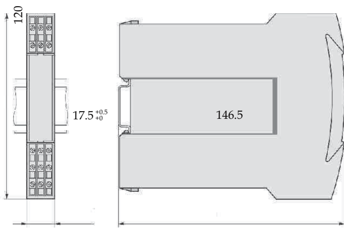
Fig. 3 Theta R in housing S 17 clipped onto a top-hat rail (35 X 15 mm or 35 X 7.5 mm, acc. to EN 50 022 ).
