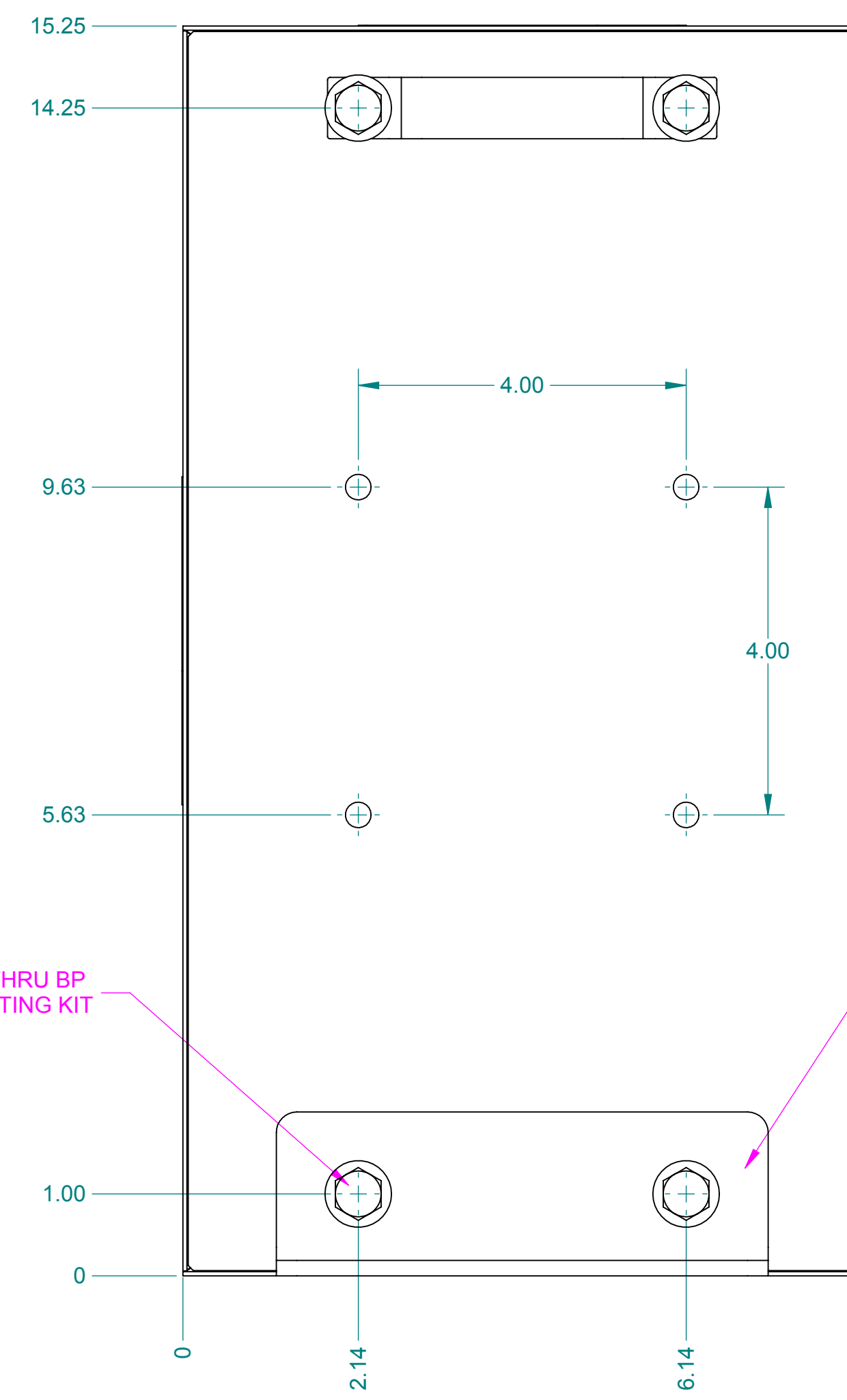
DETAIL OF ASSEMBLY SCALE:5:8
