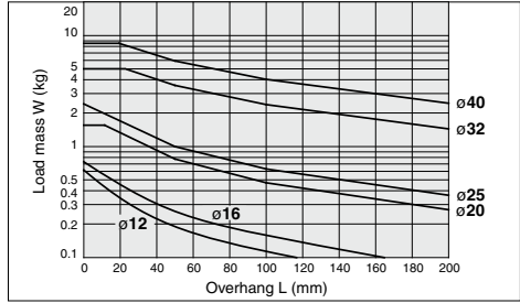
Graph (19) Stroke: Up to 100 stroke
