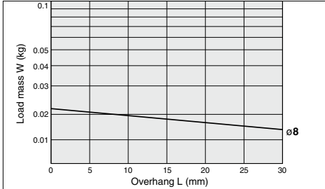
Graph (10) Stroke: Up to 30 stroke
