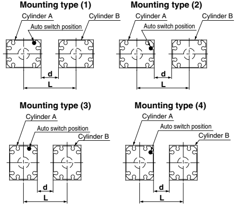
Dimensions by Mounting Type
