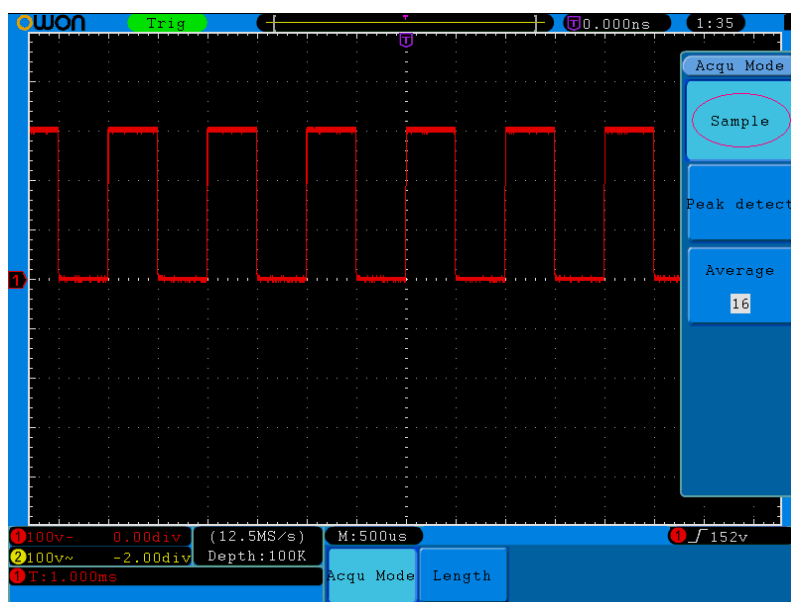
Figure 5-29 Normal ACQU Mode display, in which no burr can be detected.
