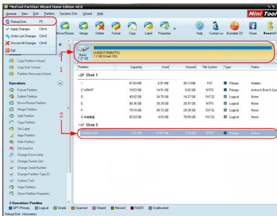
Figure 5-43: Reload Disk
