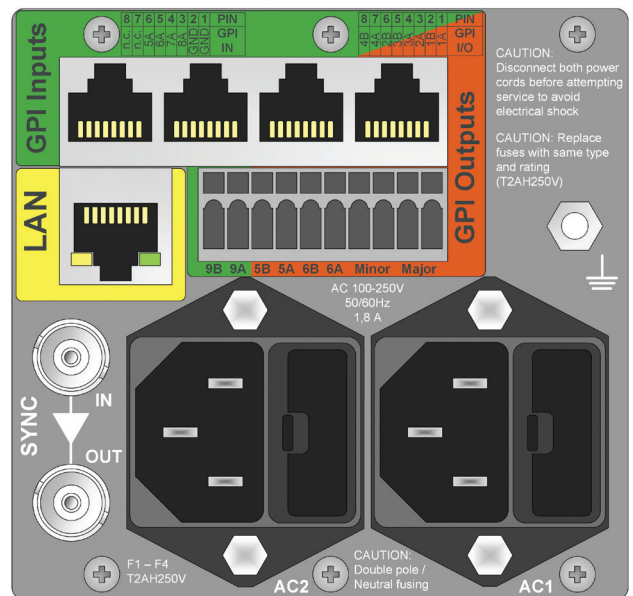
Rear Termination Panel Detail
