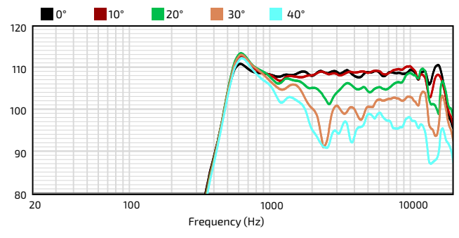
VERTICAL OFF-AXIS UP RESPONSE (dB) 10
