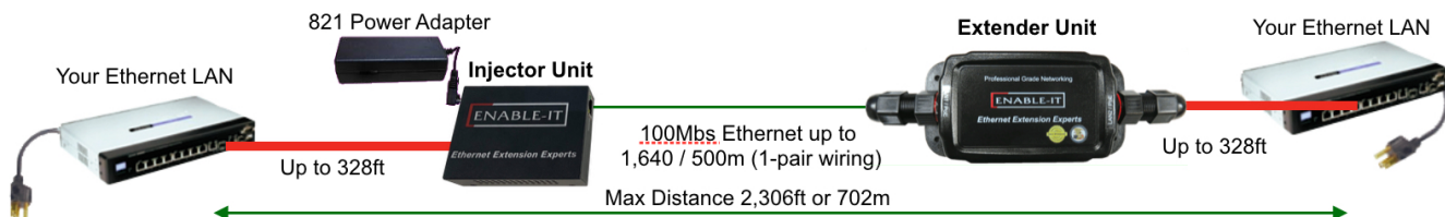
821W Outdoor Ethernet Extender
