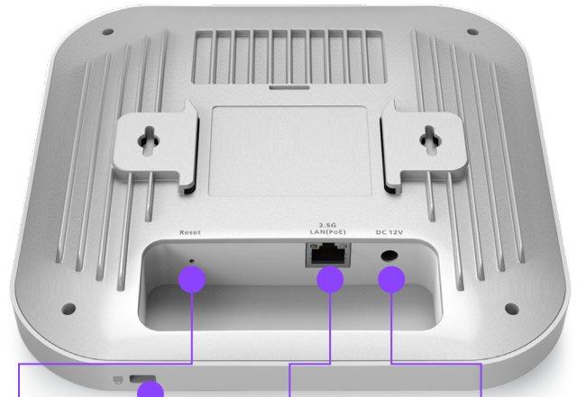
Reset Button Kensington Security Slot (PoE, 802.3af/at) 2.5Gbps LAN (PoE) Power Connector
