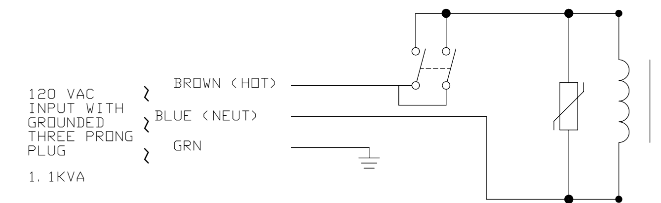
SCHEMATIC 120VAC
