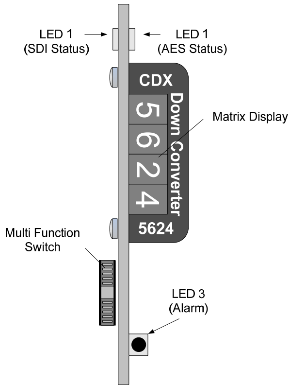
Module Front Panel
