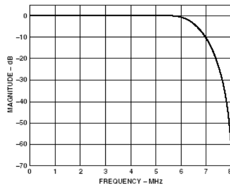
Low Pass (PAL)
